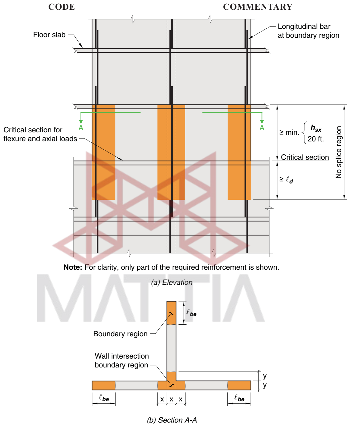
Fig. R18.10.2.3 —Wall boundary regions within heights where lap splices are not permitted.
