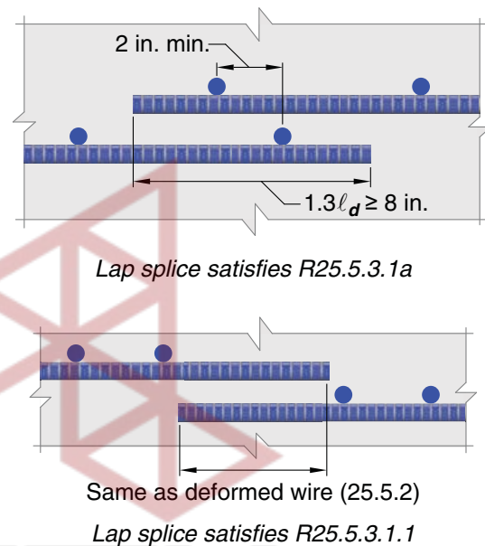
Fig. R25.5.3.1 —Lap splices of welded deformed wire reinforcement.
