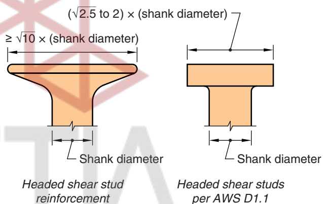
Fig. R20.4.1—Configurations of stud heads.
