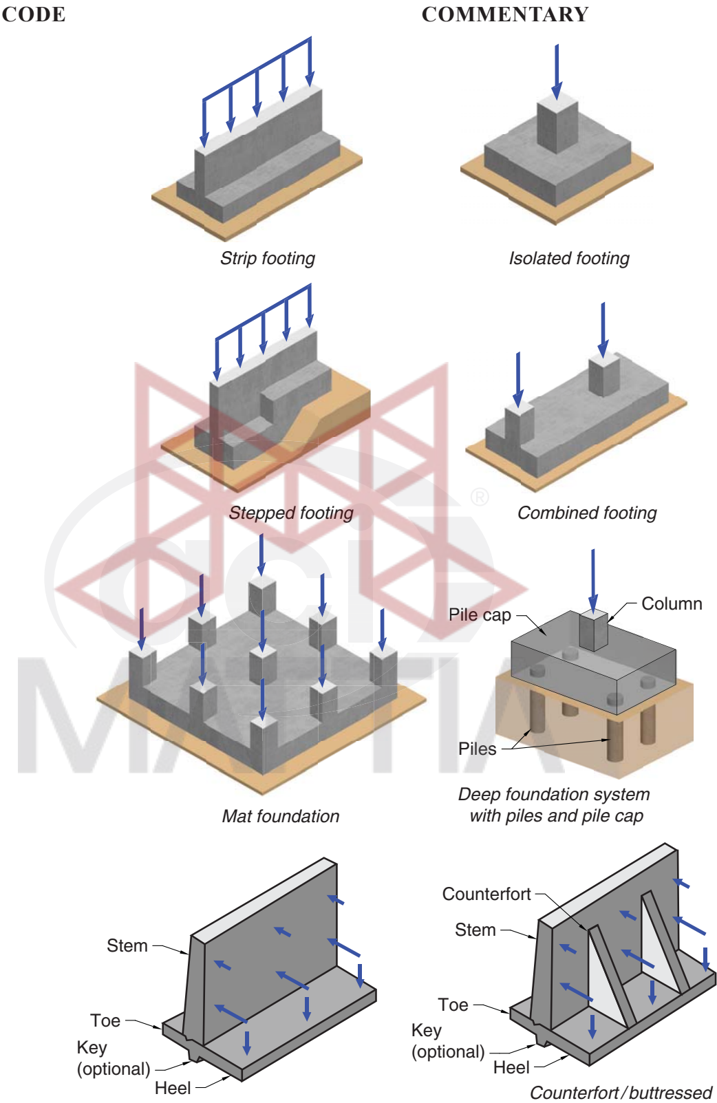
Fig. R13.1.1—Types of foundations.
