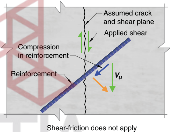
Fig. R22.9.4.3b—Compression in reinforcement.
