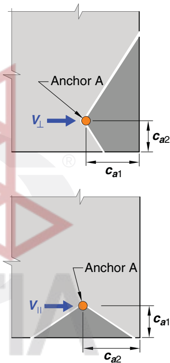
Fig. R17.7.2.1d—Shear near a corner.
