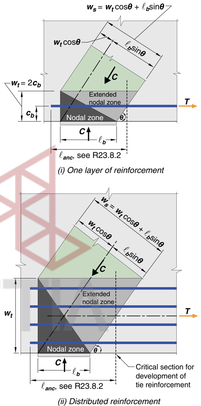
Fig. R23.2.6b—Extended nodal zone showing the effect of the distribution of the force.
