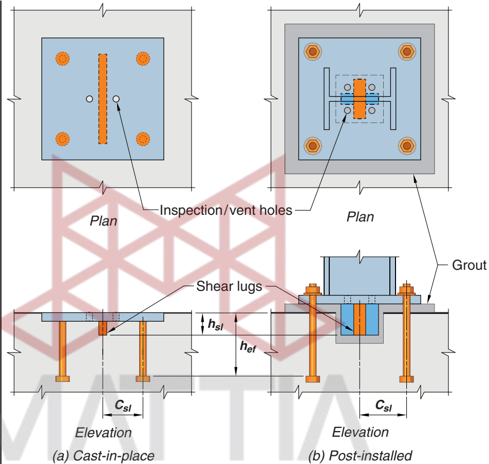
Fig. R17.11.1.1a—Examples of attachments with shear lugs.
