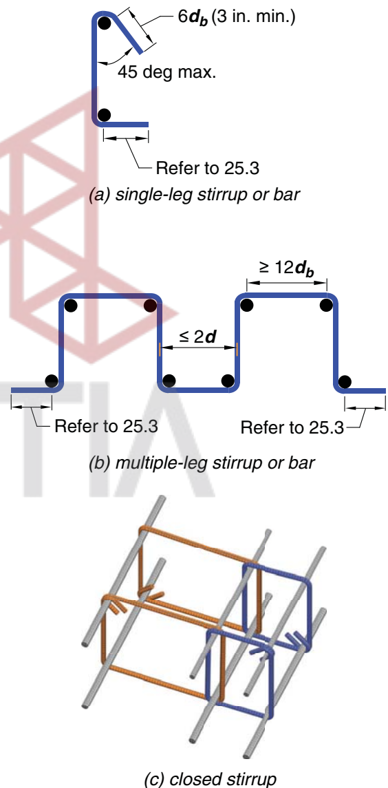
Fig. R8.7.6(a)-(c) —Single- or multiple-leg stirrup-type slab shear reinforcement.
