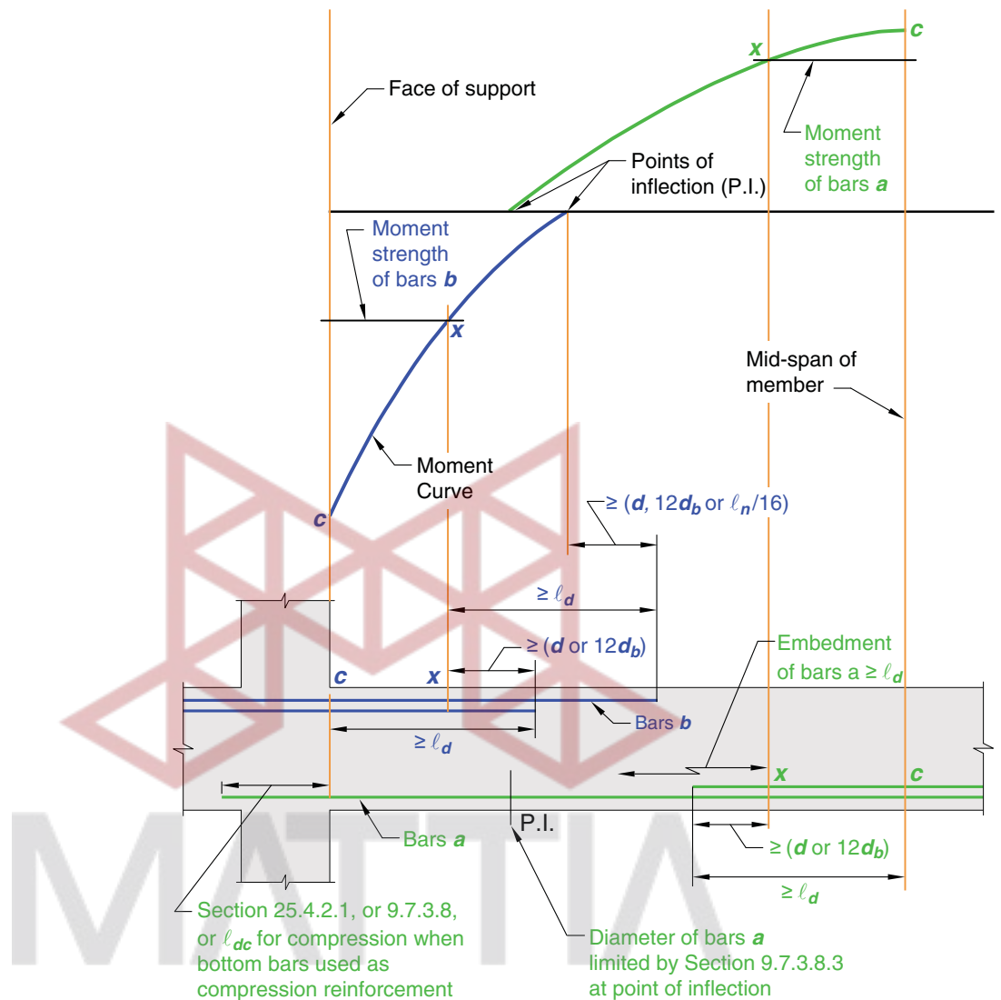
Fig. R9.7.3.2 —Development of flexural reinforcement in a typical continuous beam.
