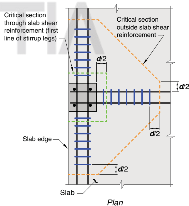
Fig. R22.6.4.2b —Critical sections for two-way shear in slab with shear reinforcement at edge column.
