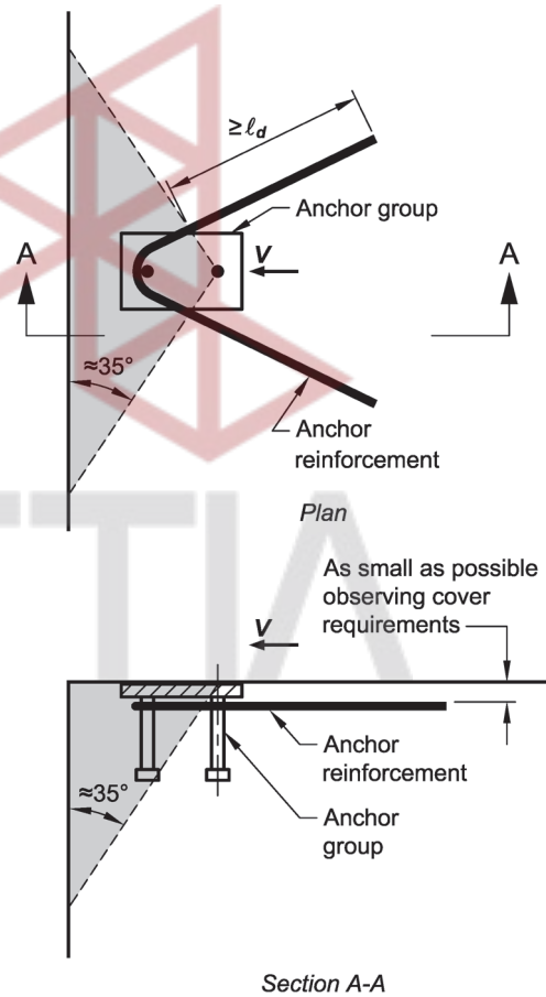
Fig. R17.5.2.9a —Hairpin anchor reinforcement for shear.
