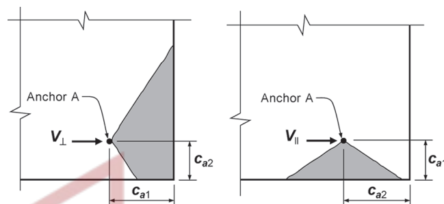
Fig. R17.5.2.1d—Shear force near a corner.
