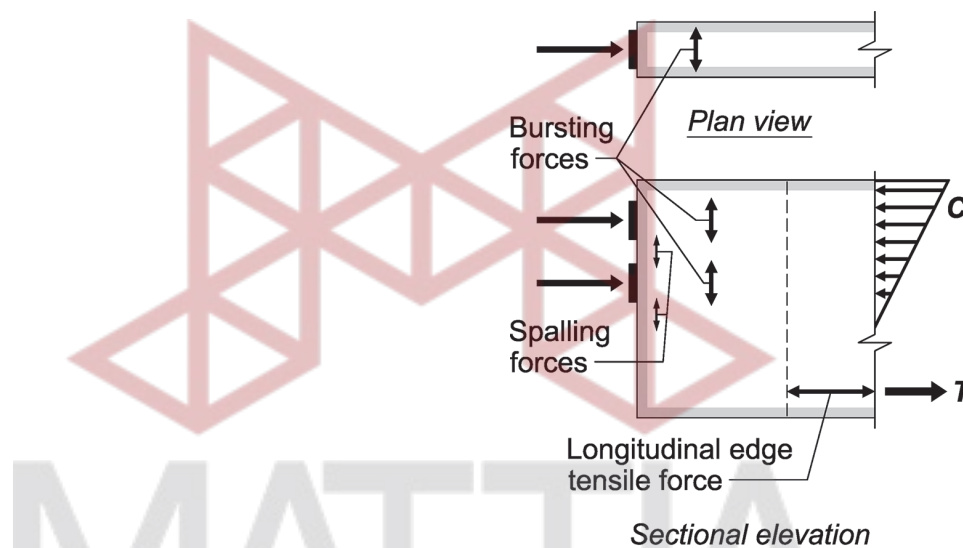
Fig. R25.9.4 —Tensile stress zones within the general zone.
