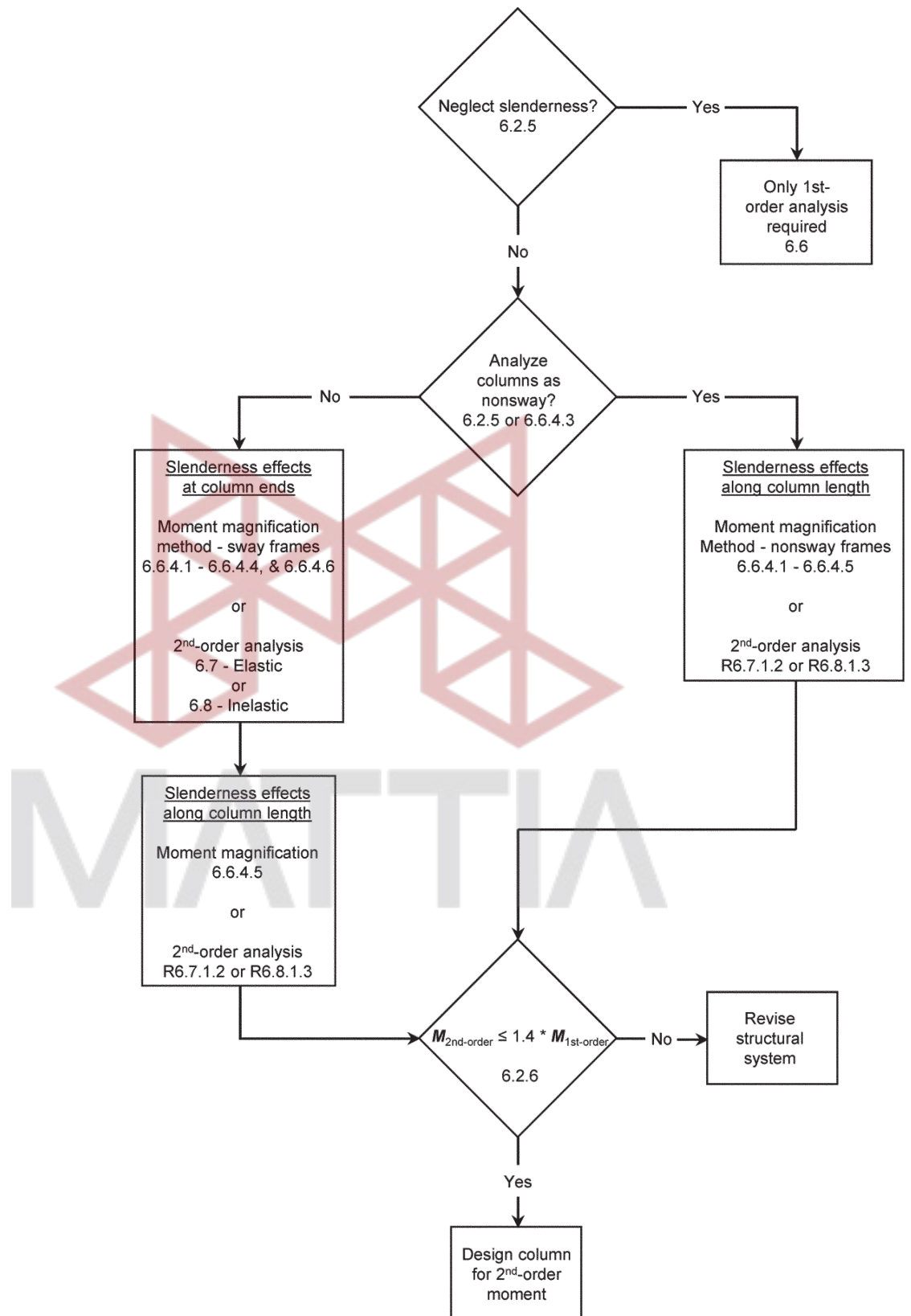
Fig. R6.2.6—Flowchart for determining column slenderness effects.
