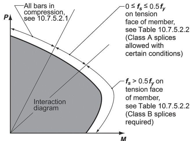
Fig. R10.7.5.2 —Lap splice requirements for columns.
