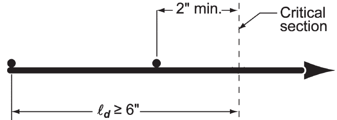
Fig. R25.4.7.2—Development of welded plain wire reinforcement.
