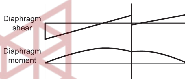
Fig. R12.4.2.3b —Diaphragm in-plane actions obtained by modeling the diaphragm as a horizontal rigid beam on flexible supports.
