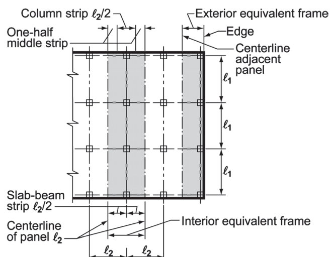
Fig. R8.11.2—Definitions of equivalent frame.
