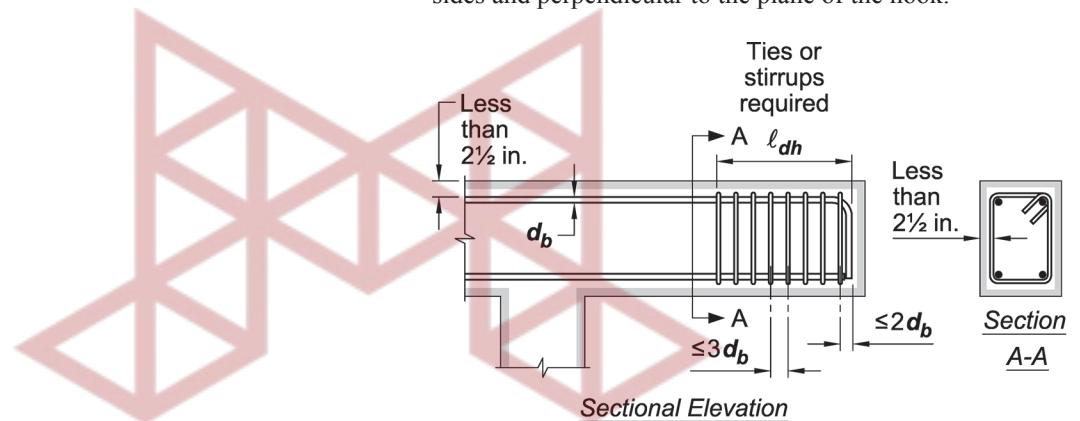
Fig. R25.4.3.3—Concrete cover according to 25.4.3.3.
