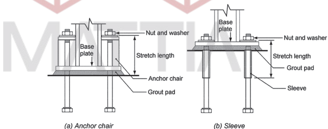
Fig. R17.2.3.4.3—Illustrations of stretch length.
