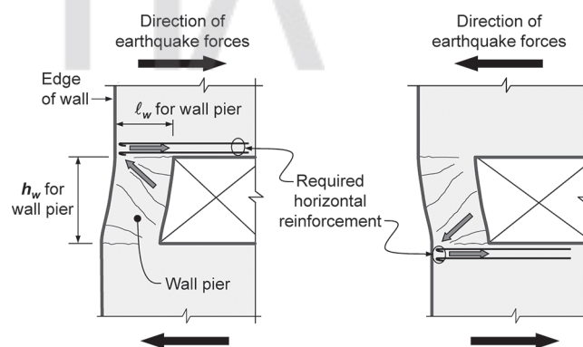
Fig R18.10.8 —Required horizontal reinforcement in wall segments above and below wall piers at the edge of a wall.
