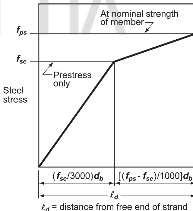
Fig. R25.4.8.3 —Idealized bilinear relationship between steel stress and distance from the free end of strand.
