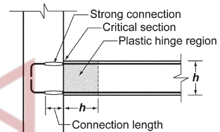
(b) Beam-to-column connection
