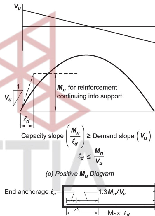
(b) Maximum \ell_d at simple support
