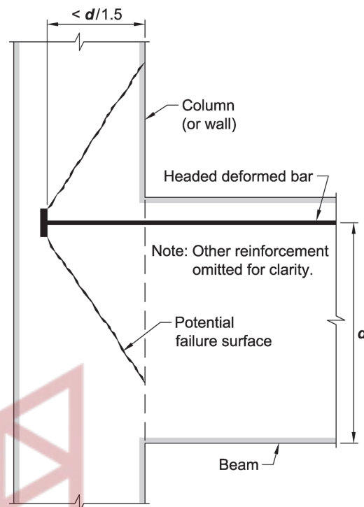
Fig. R25.4.4.2e —Breakout failure not precluded; Chapter 17 provisions applicable.
