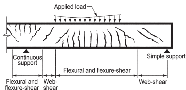
Fig. R22.5.8.3 —Types of cracking in concrete beams.
