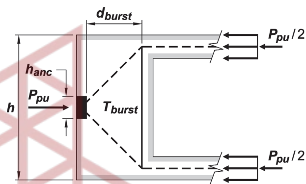
(b) Flanged section with end diaphragm
