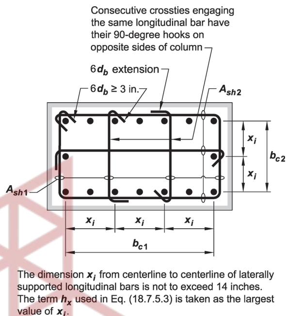
Fig. R18.7.5.2 —Example of transverse reinforcement in columns.
