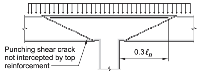
(b) Thick slab
