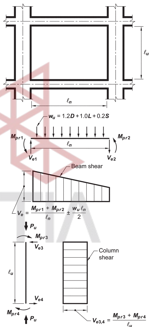
Fig. R18.6.5—Design shears for beams and columns.
