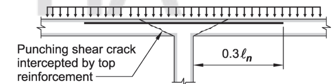
(a) Slab of normal proportions
