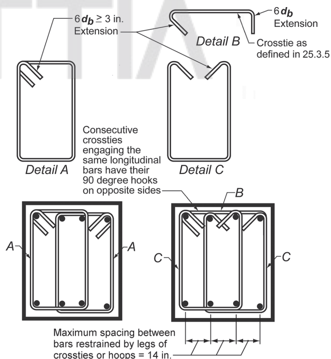
Fig. R18.6.4 —Examples of overlapping hoops and illustration of limit on maximum horizontal spacing of supported longitudinal bars.
