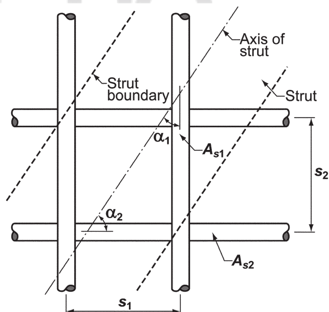
Fig. R23.5.3—Reinforcement crossing a strut.
