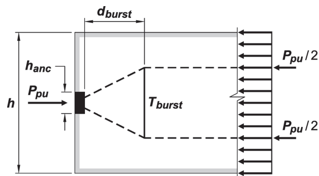
(a) Rectangular section
