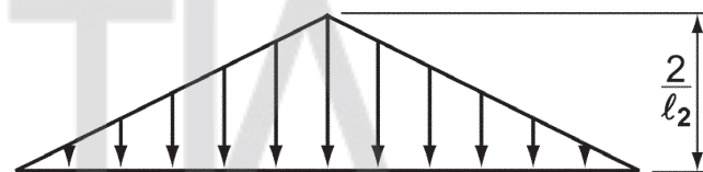
Fig. R8.11.5 —Distribution of unit twisting moment along column centerline AA shown in Fig. R8.11.4.
