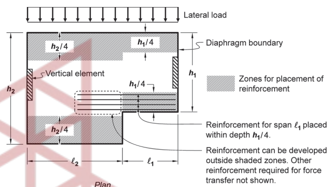
Fig. R12.5.2.3 —Locations of nonprestressed reinforcement resisting tension due to moment and axial force according to 12.5.2.3.
