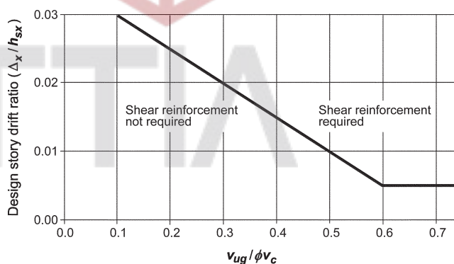
Fig. R18.14.5.1—Illustration of the criterion of 18.14.5.1.
